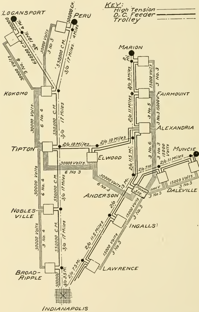
Fig. 171. Lay-Out of Power House, Substations and Transmission System Between Indianapolis and Neighboring Towns
